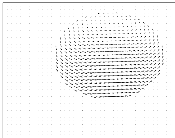
Fig. 12. A 2D field of 2D vectors representing optical flow [21] in a computer-generated rendering of a rotating sphere.
