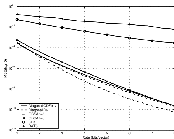
Fig. 13. Compression performance for the optical-fbw data of Fig. 12 for the VWTs used in Fig. 11.
